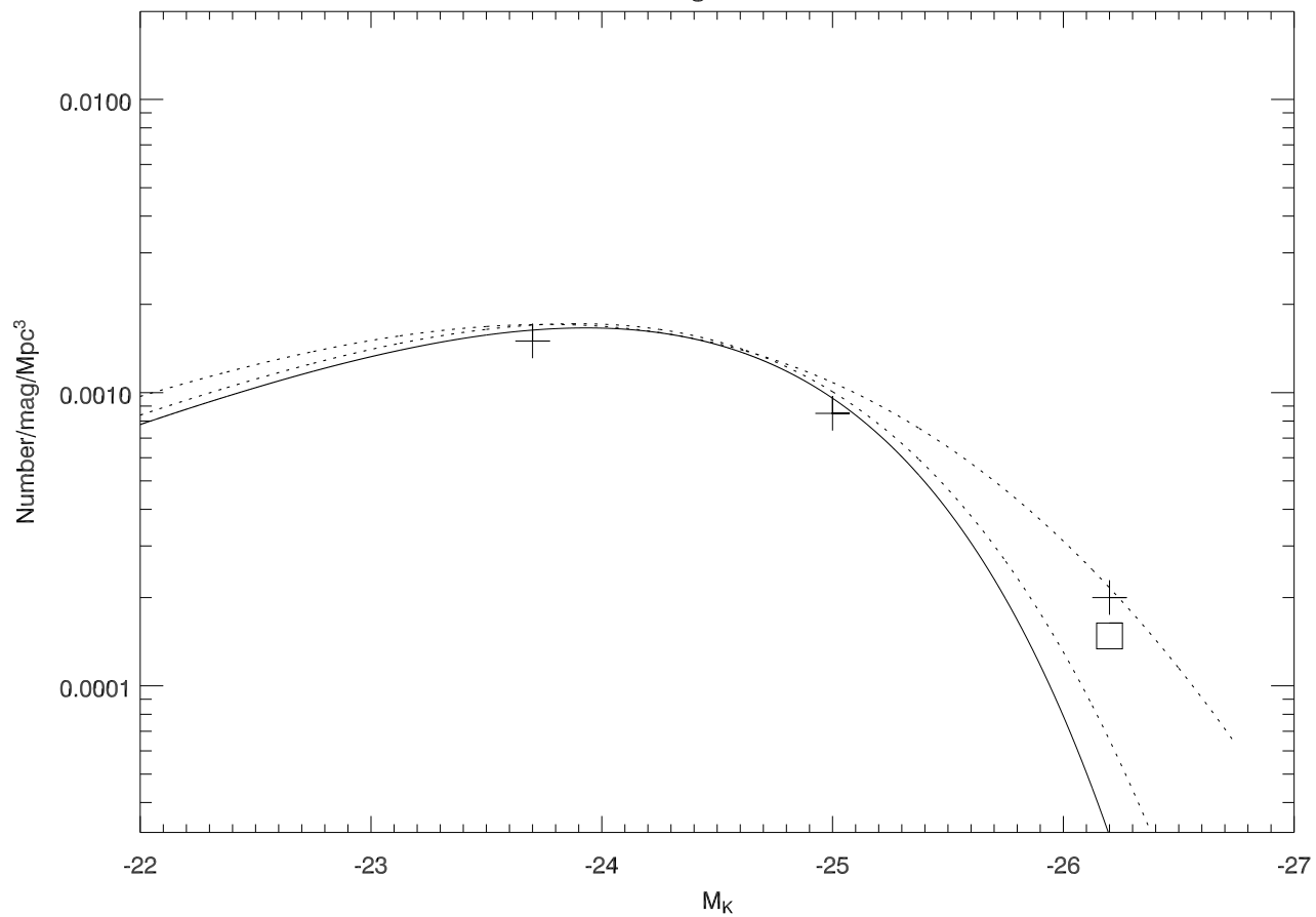
Gaussian errors in magnitude: \sigma=0.3 and \sigma=0.5
